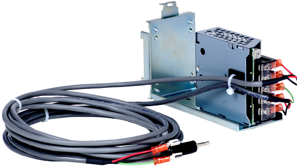
Figure 1: Mounted and Wired Power Supply
