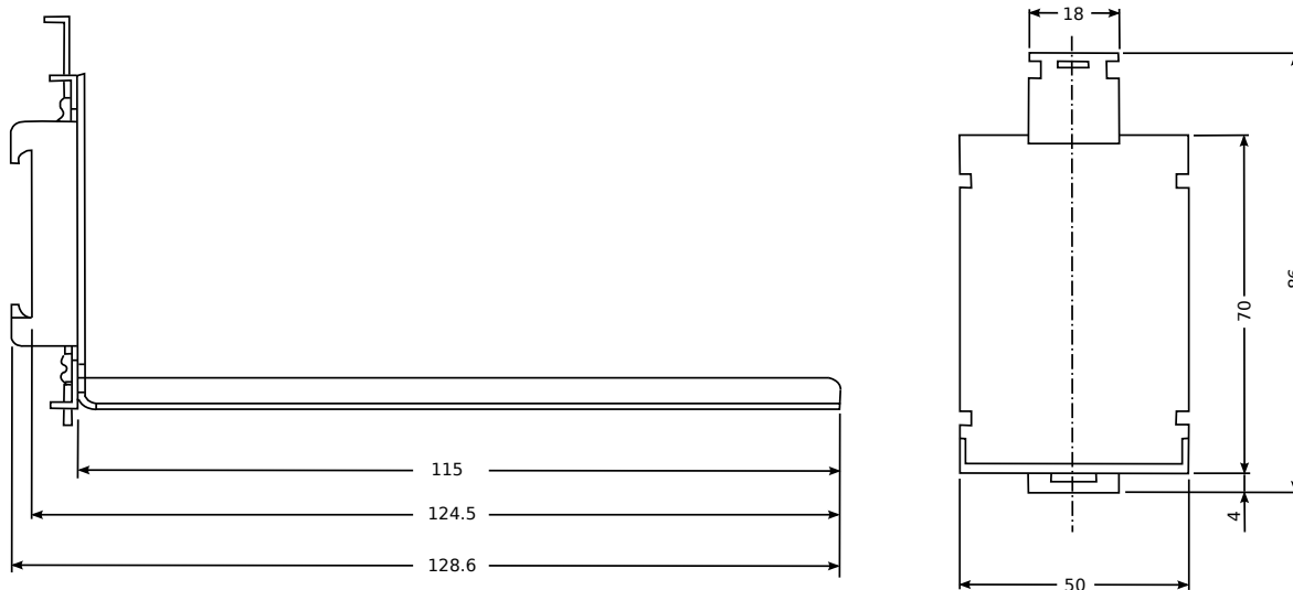
Figure 2: Attachment Plate Dimensions
