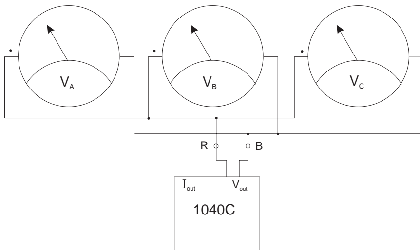
b) Meters
