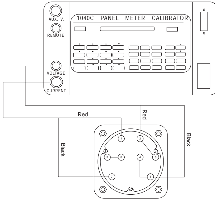
3 WIRE, 3 PHASE WATTMETER YOKOGAWA 10322 _____ 103712 _____
