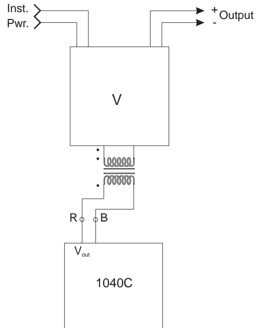
d) Voltage Transducer Calibration Connections, with Potential Transformer
