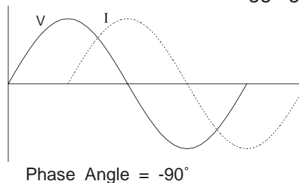
Figure 12 Phase, Power Factor, and VAR Conventions Employed by the 1040C Panel Meter Calibrator
