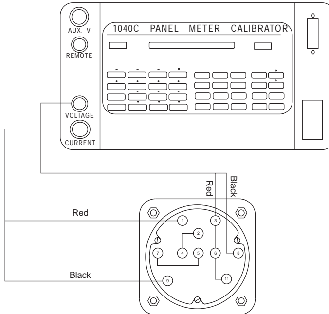
4 WIRE, 3 PHASE WATTMETER YOKOGAWA 10325 _____ 103732 _____
