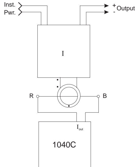
d) Current Transducer Calibration Connections, with Current Transformer
