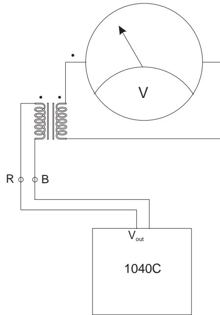
b) Voltmeter Calibration Connections, with Potential Transformer
