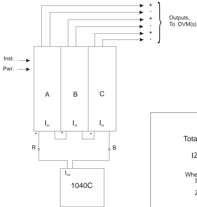
a) Transducers
